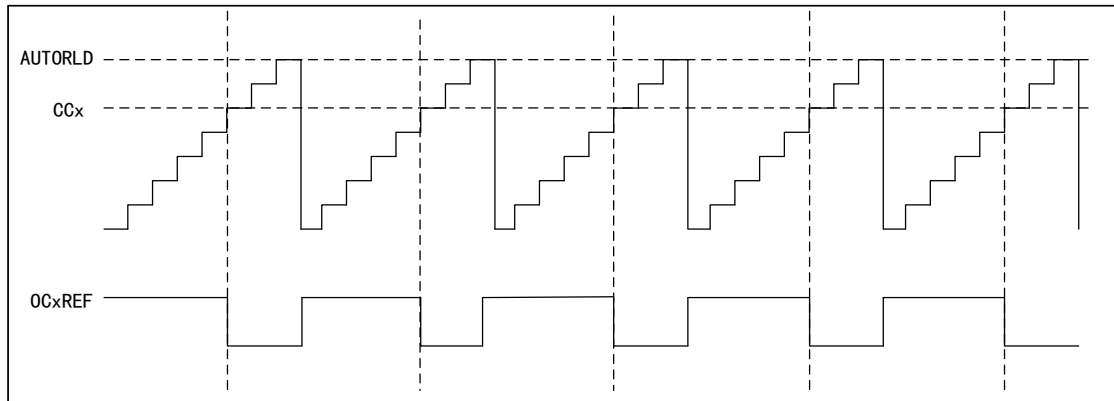
Figure 19 Timing Diagram in PWM1 Count-down Mode
