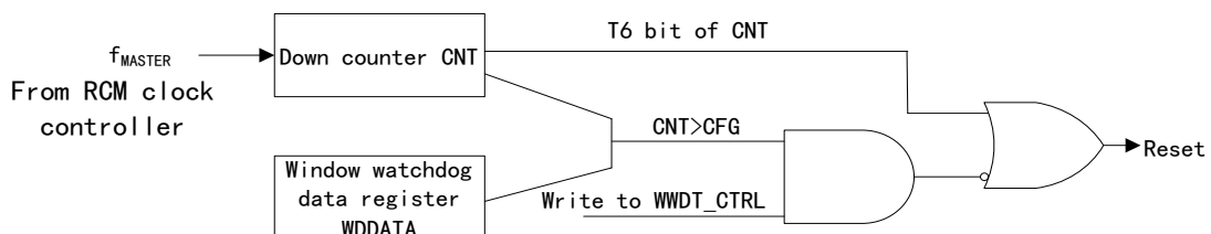
Figure 47 Window Watchdog Function Block Diagram
