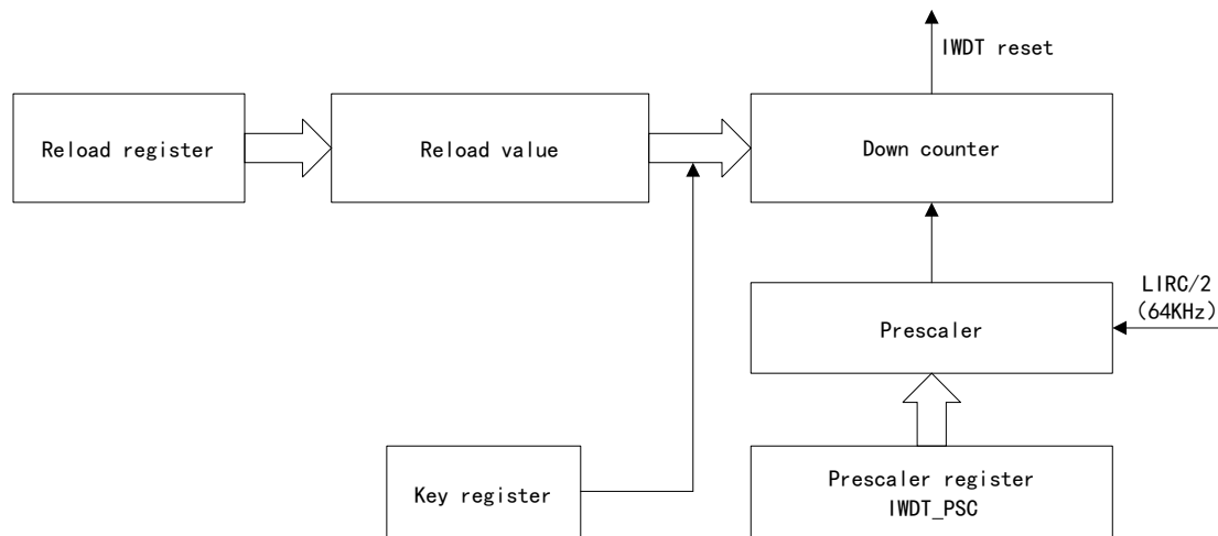
Figure 46 Independent Watchdog Block Diagram
