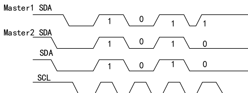
Figure 71 SDA Timing Diagram
